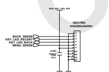
TOUCHKEY CONN
